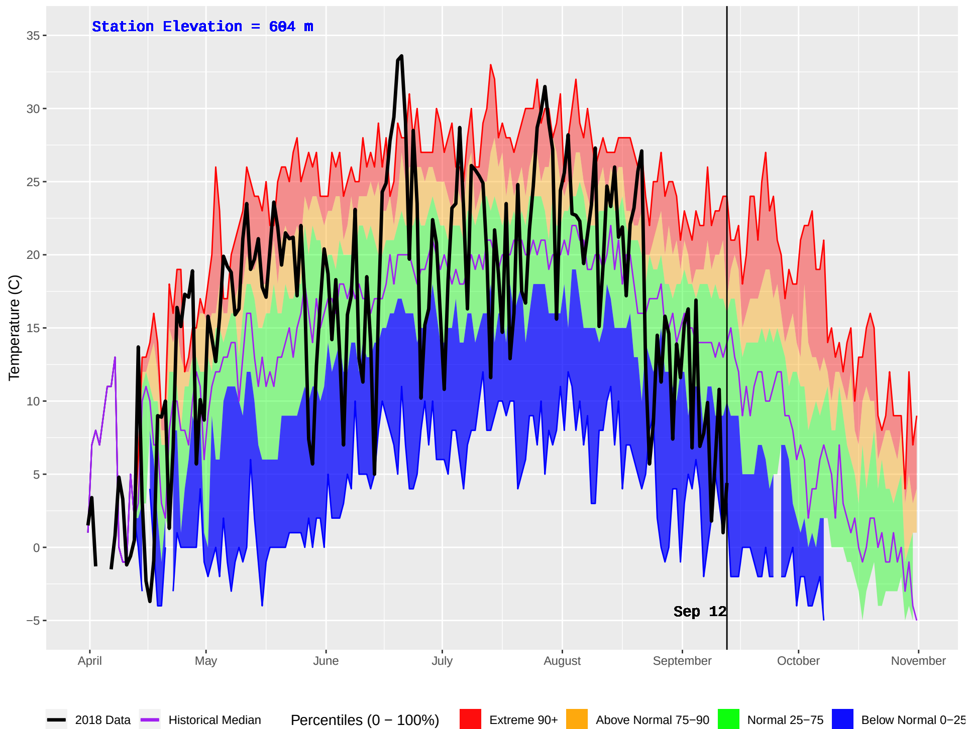
NELSON FORKS (119) : Historical (1986–2016) and Current (2018) Daily Temperature
