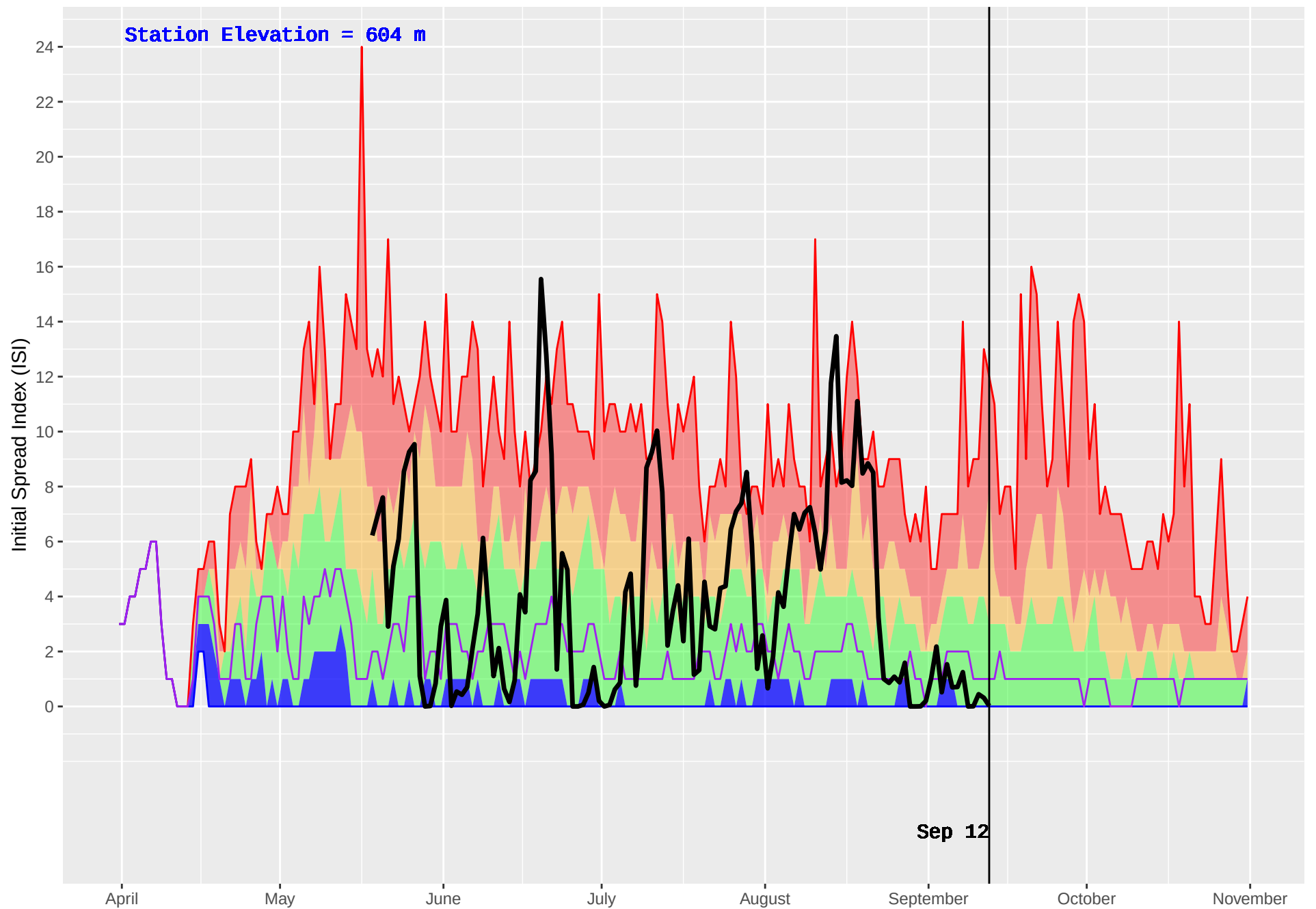
NELSON FORKS (119) : Historical (1986–2016) and Current (2018) Daily Initial Spread Index (ISI)
